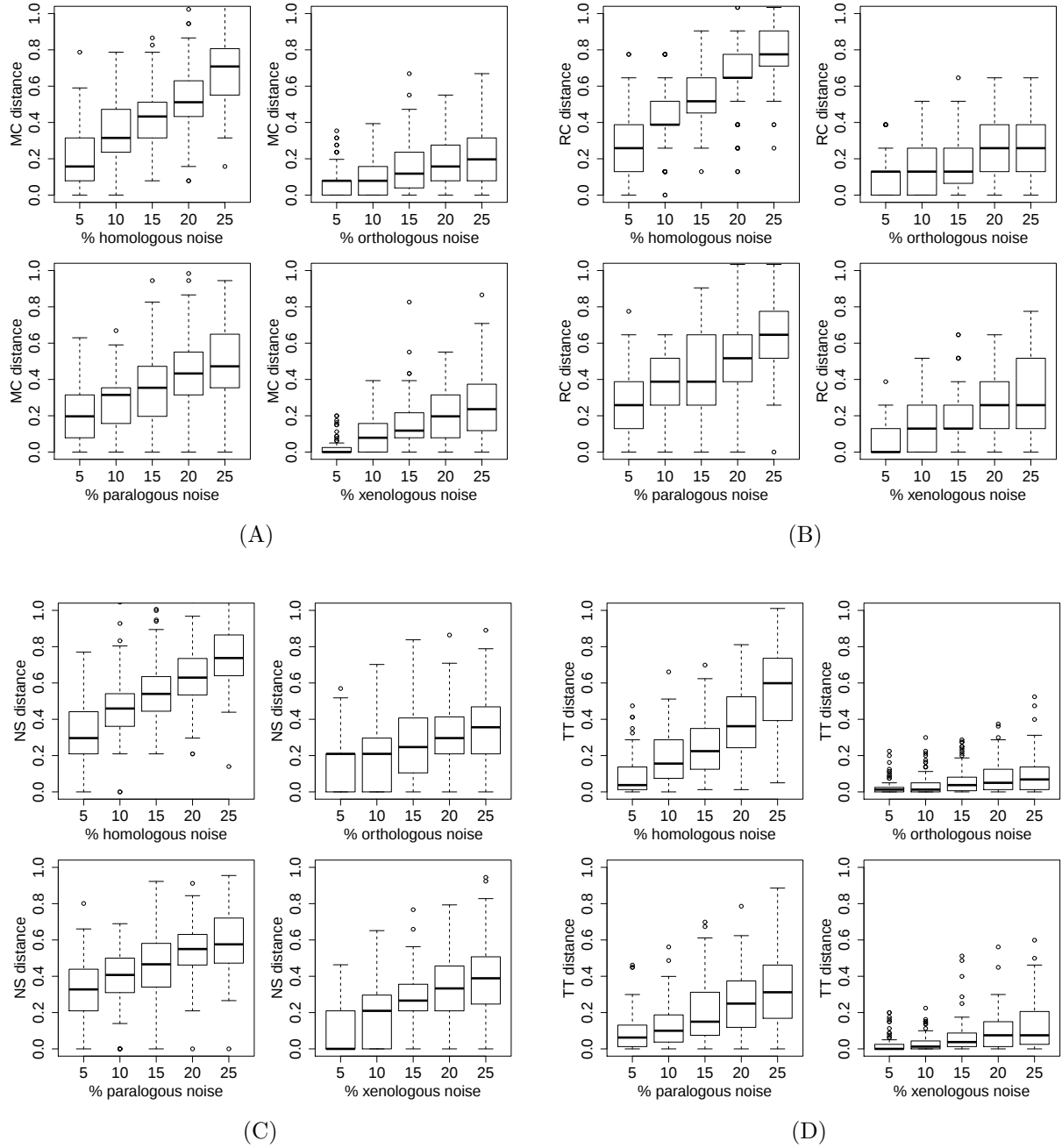
Figure S2: Matching Cluster (A), Robinson-Foulds (B), Nodal Splitted (C) and Triple metric (D) tree distances of 100 reconstructed phylogenetic trees with ten species. For each model noise was added with a probability of 0.05 to 0.25.
