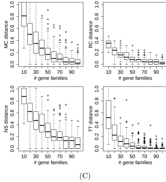
Figure S1: Matching Cluster (MC), Robinson-Foulds (RC), Nodal Splitted (NS) and Triple metric (TT) tree distances of 100 reconstructed phylogenetic trees with five (A), ten (B), and 15 (C) species and ten to 100 gene families, each.
