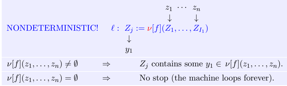
Figure 5: Oracle instruction with \nu -operator
