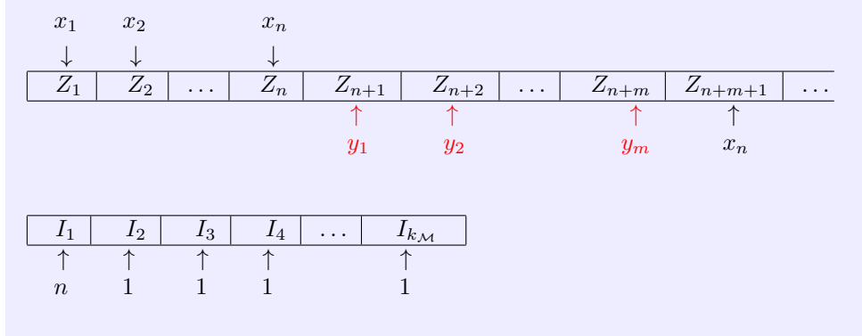
Figure 3: Guessing by an input-guessing procedure of nondeterministic machines
