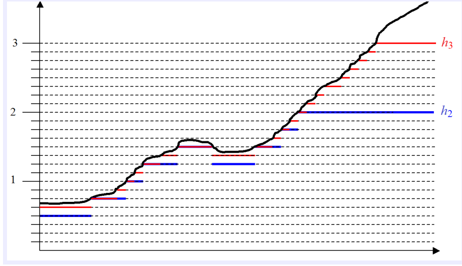
Figure 7: The simple functions h_n
