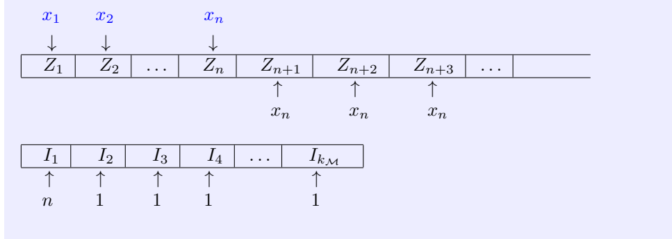
Figure 2: The input of x_1, \dots, x_n by an input procedure of any deterministic BSS RAM
