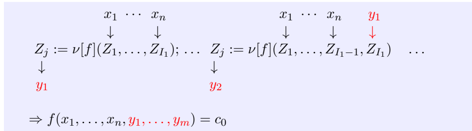
Figure 6: Guessing by the \nu -operator of a \nu -oracle machine
