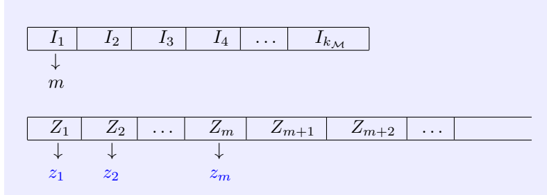
Figure 4: Output procedure of any BSS RAM
